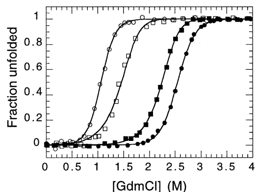
Figure 2. Normalized transition curves for the stabilized monomeric V L domain V L -601 (circles) and the homodimeric IcaL-14 (squares) at 20°C and pH 7.4. Filled symbols refer to oxidized domains (intact disulfide bridge), open symbols to reduced domains (free thiols). Protein concentrations were 2 μM referring to the monomer. Both domains fold fully reversibly under oxidizing and reducing conditions.
