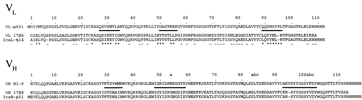
Figure 1. Sequences for the variable domains used in this study: V L -μ601 and the catalytic intrabody Ica-Fv, and the variable domains of the antibody 17E8. CDRs of 17E8 are underlined, changes introduced into the respective framework sequences for grafting the catalytic epitopes are indicated with an asterisk (*), the remaining sequence differences between the catalytic 17E8 and Ica-Fv are emphasized with a (~). IcaL-η14 deviates in 29 positions, IcaH-μ01 deviates in 17 positions from the 17E8 sequence.
