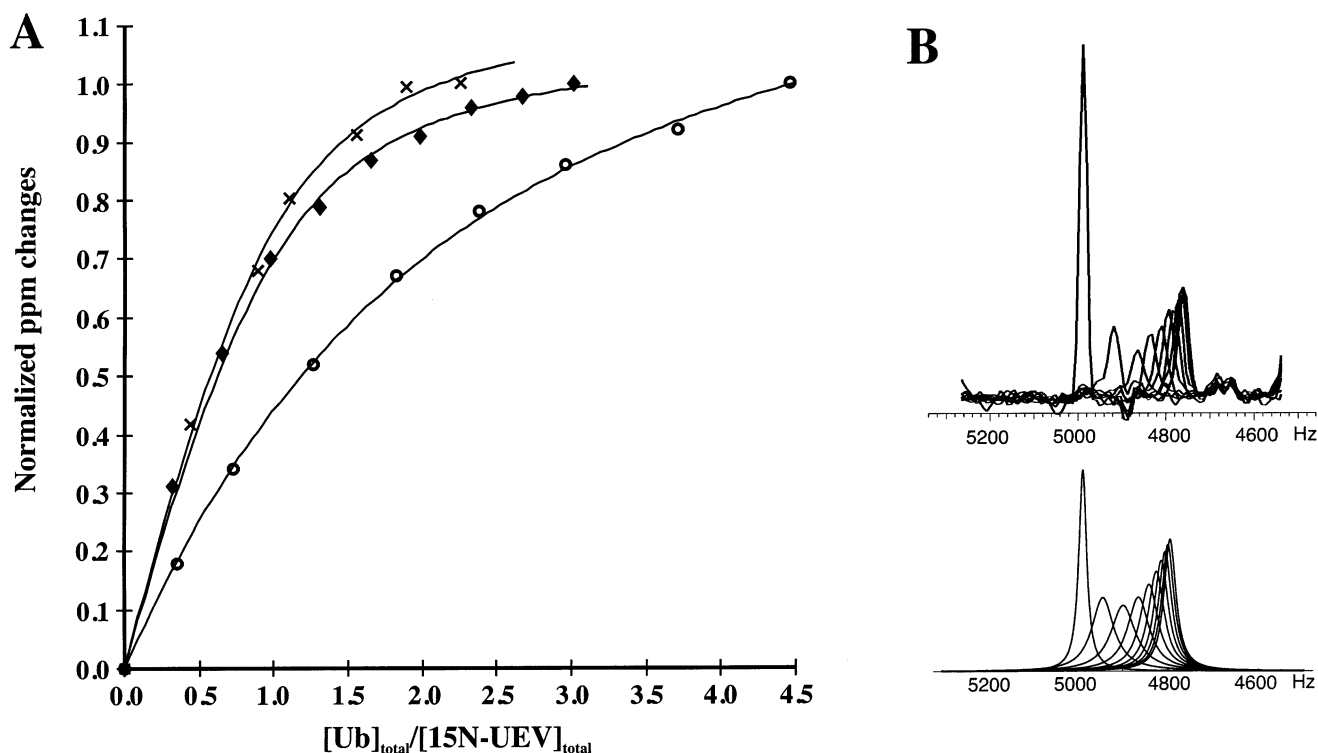
FIGURE 3: (A) Binding curves derived from 2D ^1\text{H} - ^{15}\text{N} HSQC NMR titrations of Ub into [ ^{15}\text{N} ]Mms2 ( \blacklozenge ), [ ^{15}\text{N} ]Uev1a (O), and [ ^{15}\text{N} ]-Mms2·Ubc13 ( \times ). The average normalized changes (parts per million) are plotted as a function of the [\text{Ub}]/[^{15}\text{N}\text{-labeled species}] ratio, with nonlinear least-squares fits to the data shown as solid lines. The errors in the data points are smaller than the size of the corresponding symbols. (B) 1D ^1\text{H} traces taken through the cross-peaks of Val ^{26} from 2D ^1\text{H} - ^{15}\text{N} HSQC NMR spectra during titration of Ub into [ ^{15}\text{N} ]-Mms2 (top). The corresponding line shape simulation using a k_{\text{off}} value of 2250 \text{s}^{-1} is also shown (bottom).
