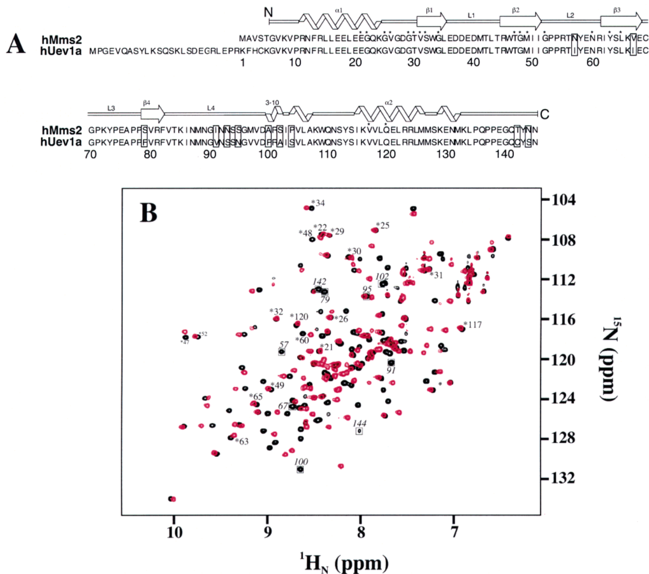
FIGURE 4: (A) Sequence alignment of human Mms2 and Uev1a, shown with the corresponding secondary structures (24). Important residues are labeled as described below. (B) Superposition of 2D 1 H– 15 N HSQC NMR spectra of free [ 15 N]Mms2 (black) and [ 15 N]Uev1a (red). Cross-peaks in [ 15 N]Mms2 which are affected by complex formation with Ub are numbered and denoted with an asterisk, while those which differ between the UeVs are numbered and boxed.
